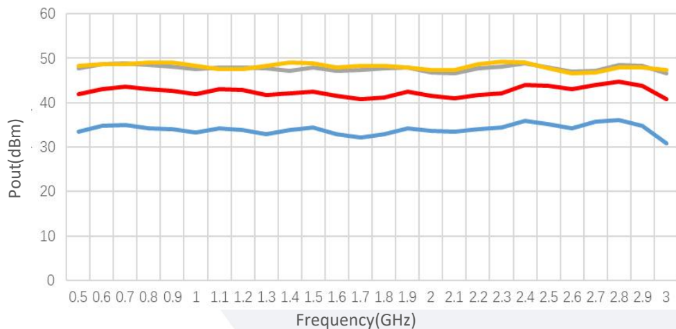
Pout@Equal_Pin
