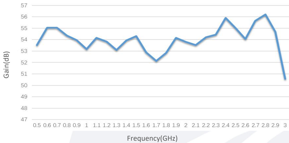
Pout@Equal_Pin
