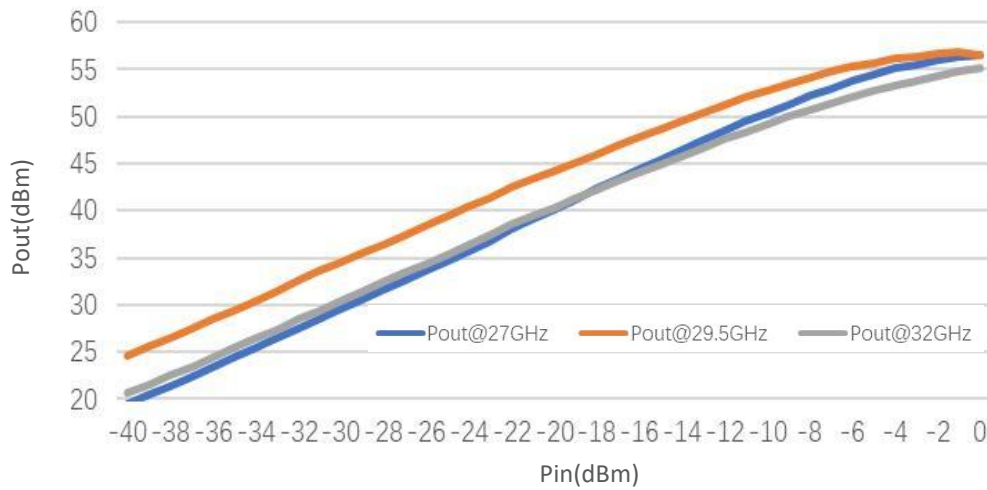
Pout@Equal_Pin
